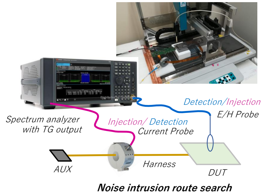
BCI measurement environment
